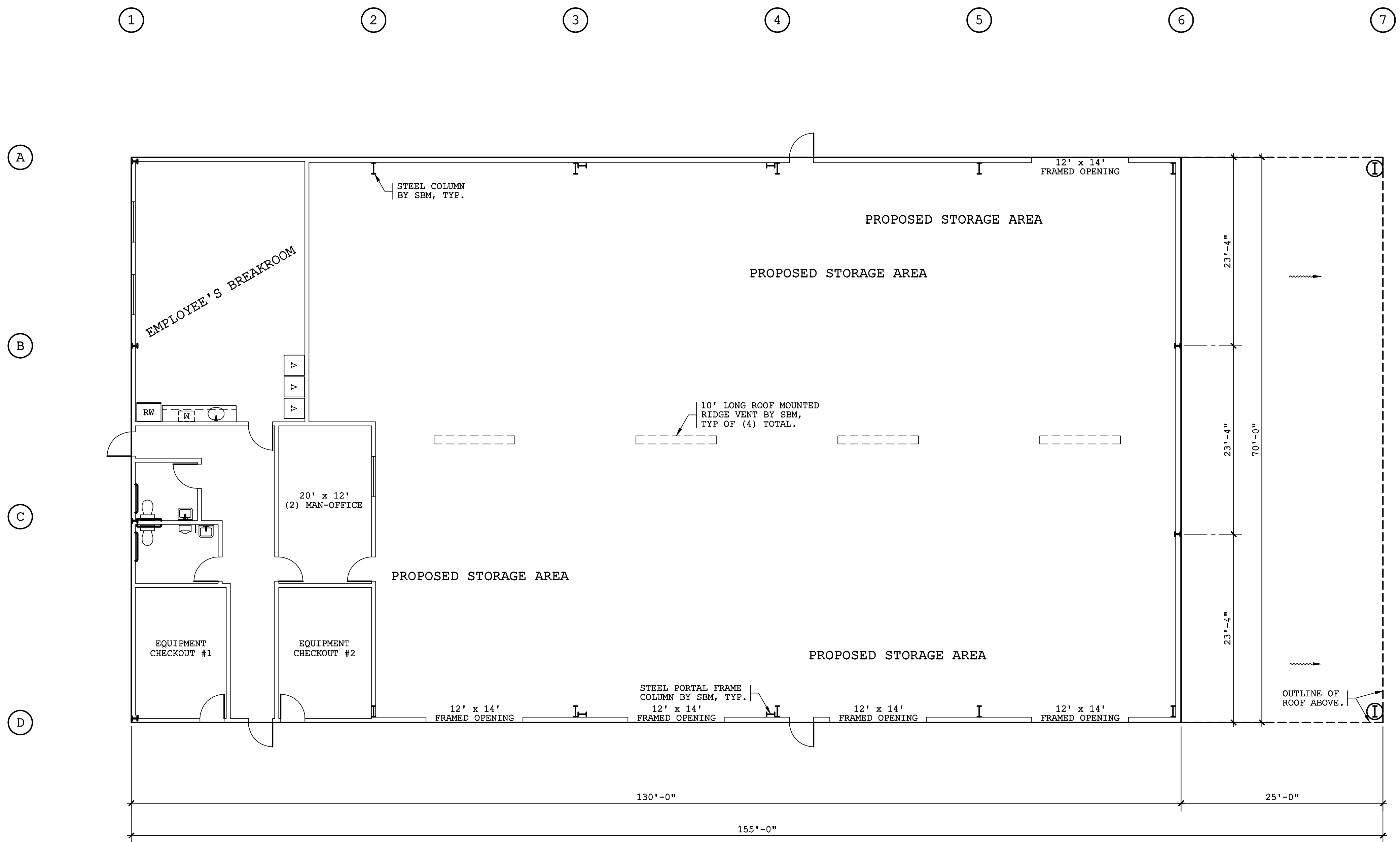
BUILDING #2'S FLOOR PLAN NORTH REF. SCALE: 1/8" = 1'-0"
