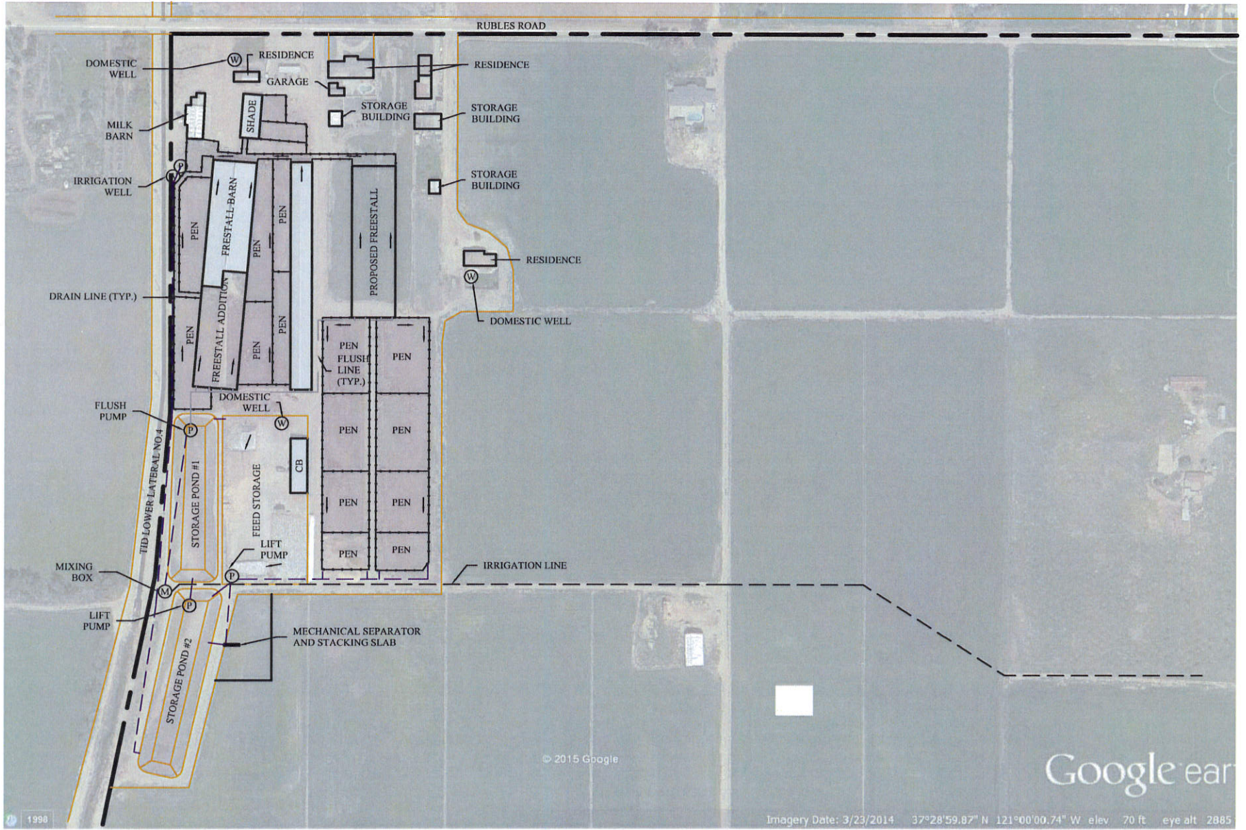
FIGURE 2 Proposed Site Plan KR Blount-fields and Facility
